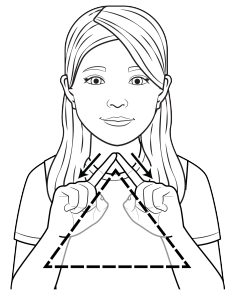
triangle
