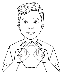
hexagon
