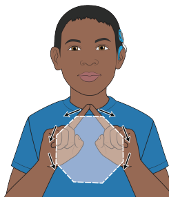
octagon
