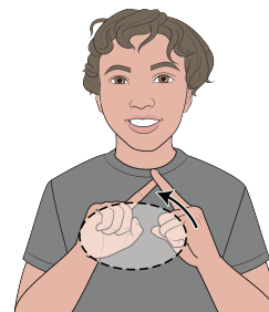
oval
