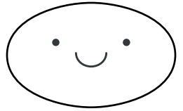
oval
