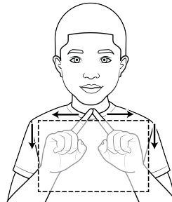
rectangle
