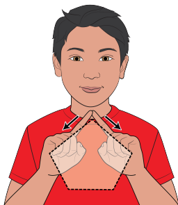
pentagon
