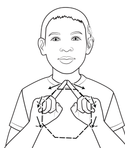
octagon
