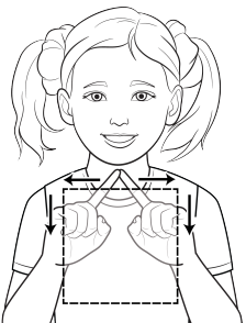
square
