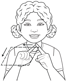
parallelogram
