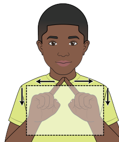
rectangle
