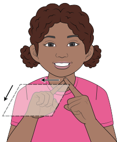
parallelogram
