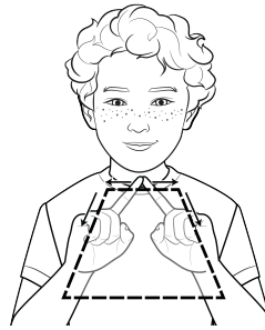
trapezoid
